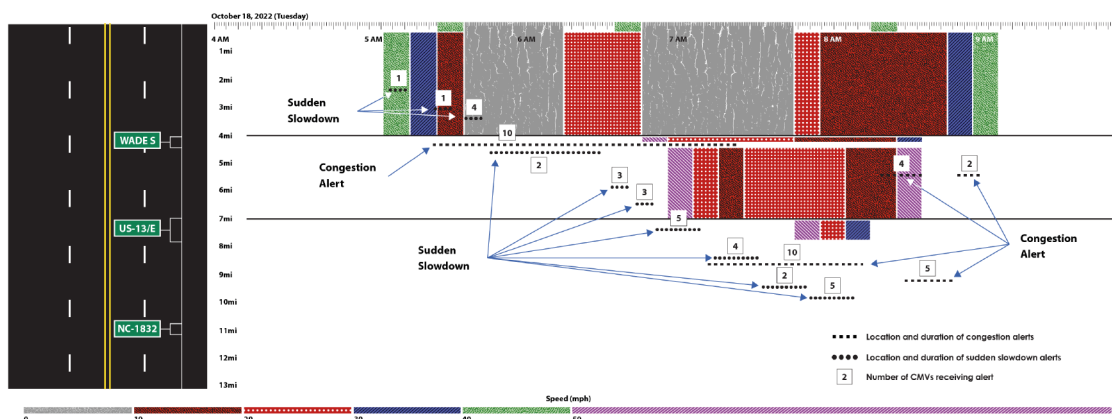
Source: North Carolina Department of Transportation (NCDOT). Figure 3. Illustration. Correlation of speed heatmap and commercial motor vehicle electronic logging devices' sudden slowdown and congestion ahead warning messages.
