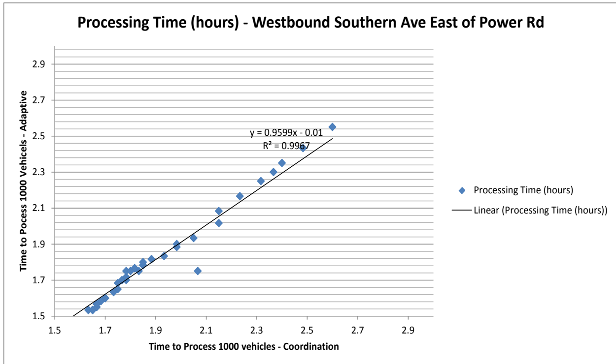
Figure 68. Line Graph. Throughput Performance for ASCT versus Coordination – Volume Counter “B”, Westbound (Source: Kimley-Horn and Associates, Inc.)
